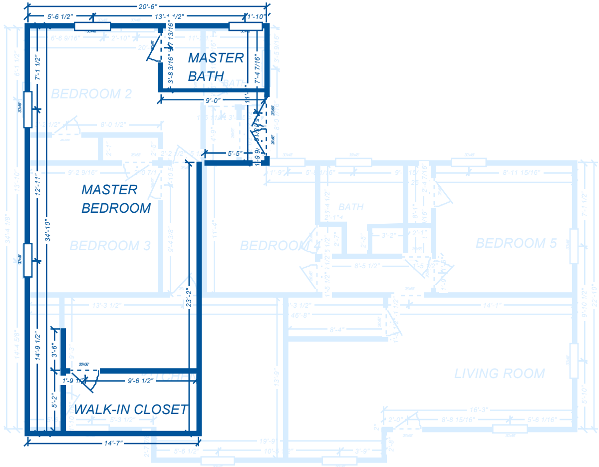
FLOOR 2
